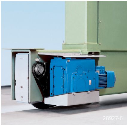
Angular gearbox operating outdoors as a cleaning machine drive
