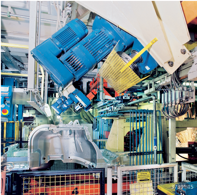
Drive for starting and stopping applications with short cycle times and high positioning accuracy in an automotive welding line
