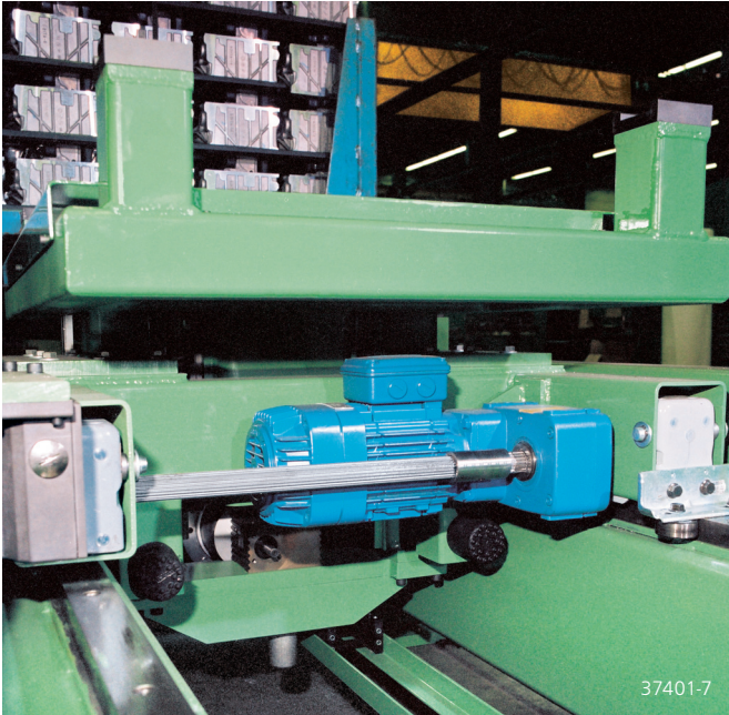
Line-fed KBF motor used as a shuttle drive for smoothly transporting goods in a storage system
