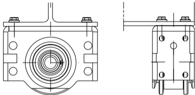
Top connection
